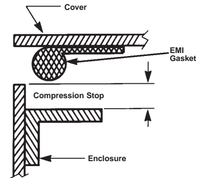
Figure 5b. Compression Stop Built into Enclosure
