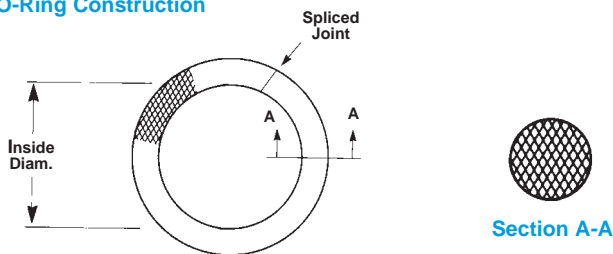
Figure 2. O-Ring Construction
