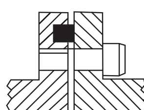
Figure 4. Mounted in Flange Groove
