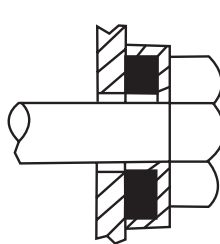
Figure 3. With Positive Stop Cup Washer
